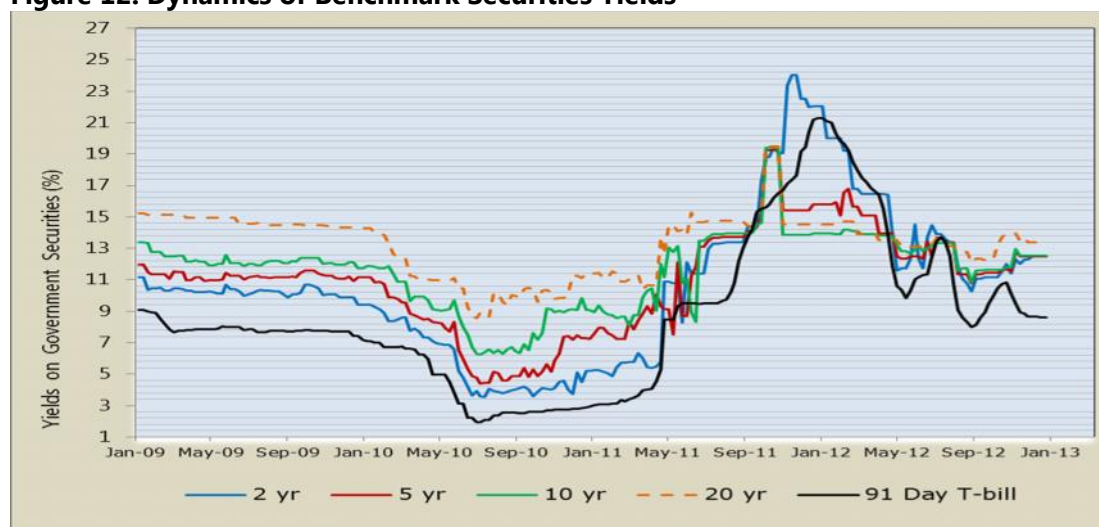
Figure 12: Dynamics of Benchmark Securities Yields
