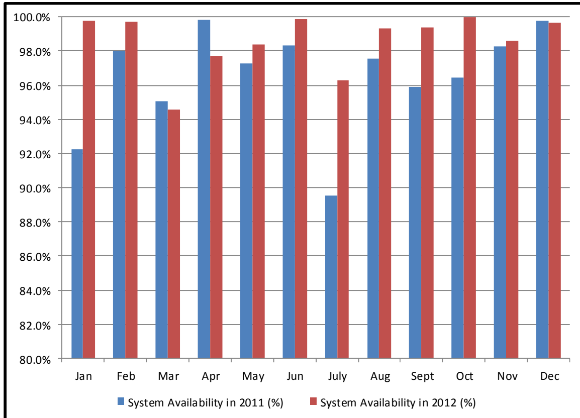
Figure 20: KEPSS Availability
